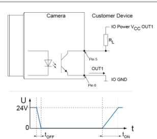
Digital Output: Low Active
