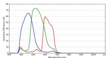
MV-CE200-10UC Quantum Efficiency
