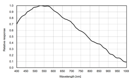
MV-CE200-10UM Quantum Efficiency
