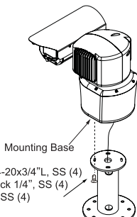
Pedestal Mount*
