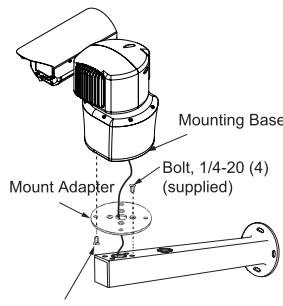
Wall Mount 8425-7
