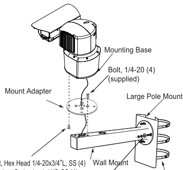
Pole Mount 8503-0
